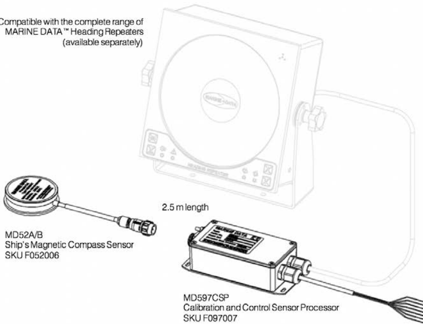
MD52A/B sensor mounts underneath the ship's compass bowl using mounting MD54 or MD58 (available separately, depending on the host compass type)
